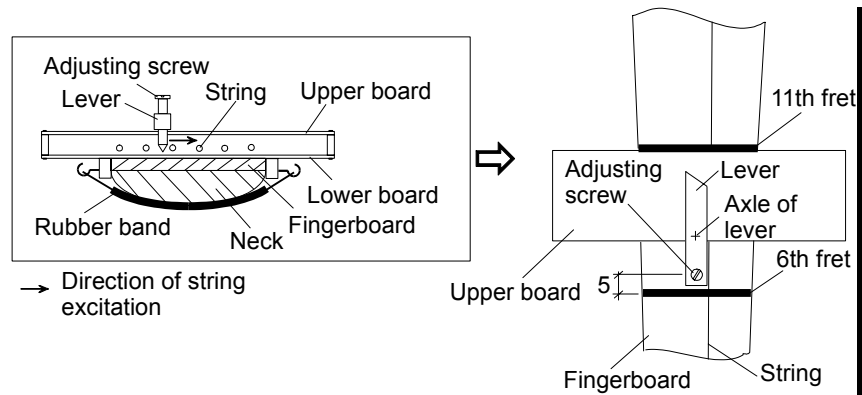
Figure 6. The string excitation device and its mounting.
