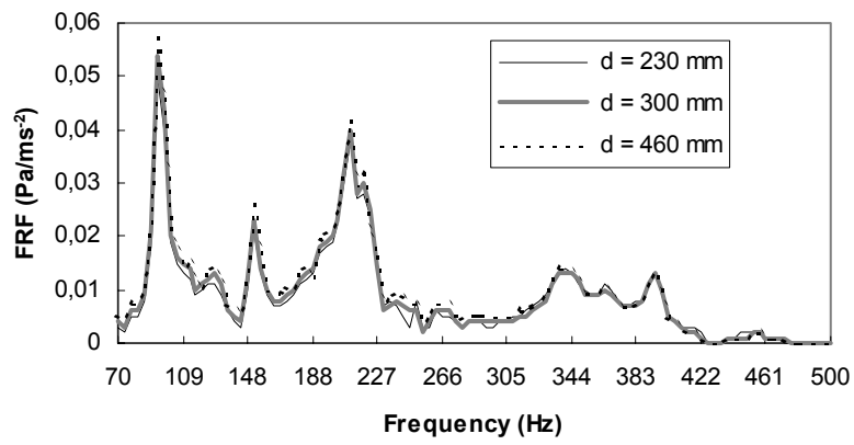
Figure 4. The FRF in dependence on d (bad guitar).
