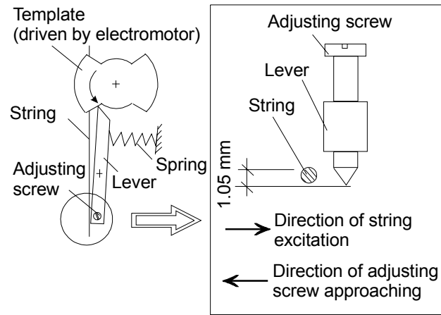
Figure 7. The operation of string excitation device (schematically).
